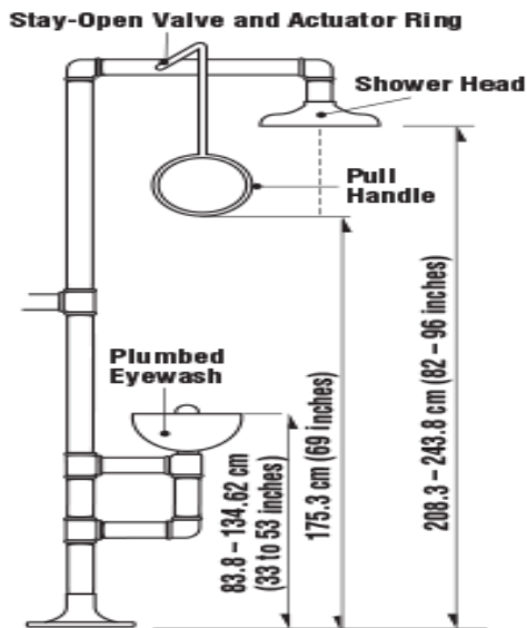
Fig.1 Shower Station
