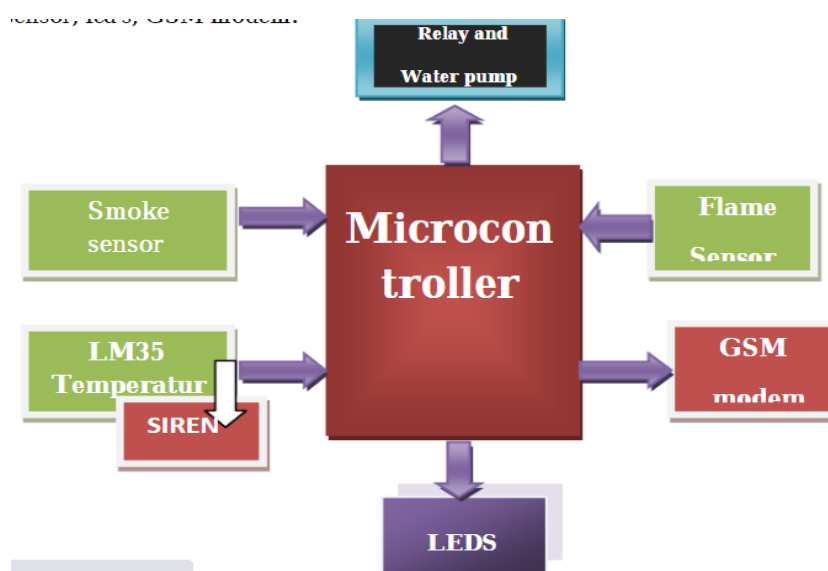
Block diagram of the wireless fire fighting system
